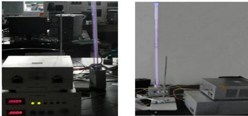
Fig. (1). The unipolar incentive column plasma antenna.
