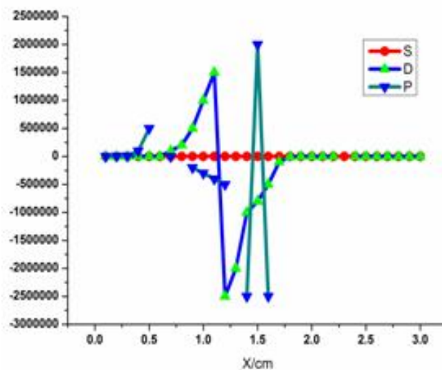
Fig. (7). The dielectric tensor when incentive power is 30W and frequency is 35MHz.
